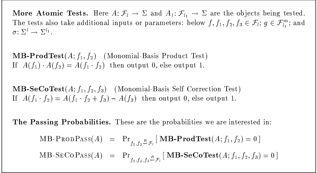
Figure 3.9: More atomic tests and their passing probabilities.
