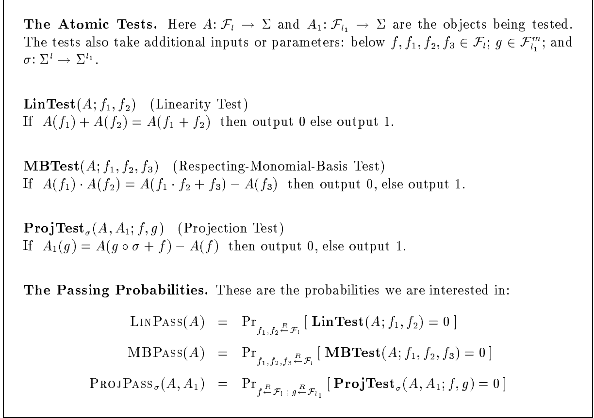
Figure 3.2: The atomic tests and their passing probabilities.
