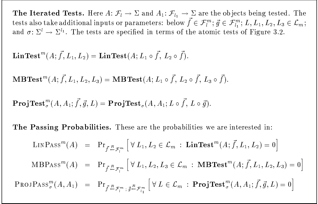
Figure 3.12: The iterated tests and their passing probabilities.
