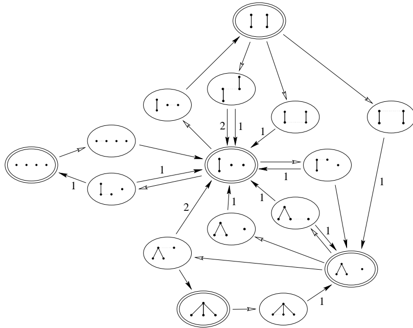
Figure 4: A mean payoff game that corresponds to the problem of selecting the second largest element with only four storage locations.
