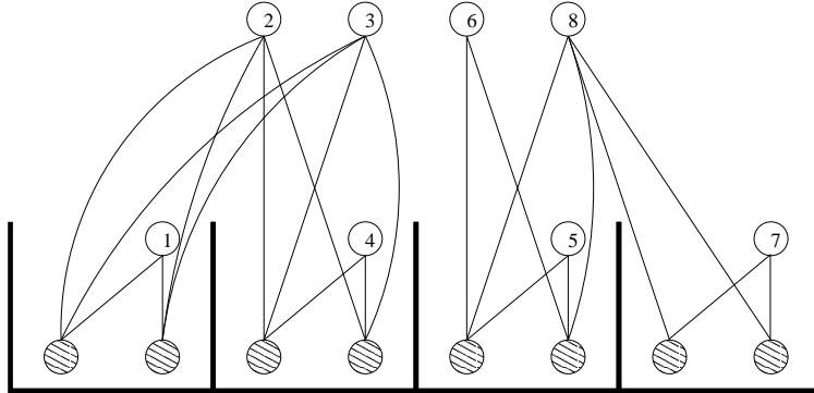
Figure 3: The vertices \{1, 4, 5, 7\} are the randomly chosen roots. In the figure we see the right assignment of these vertices to the boxes. For all the neighbors of the special vertices we know the area of at most 3 boxes, where they belong to.
