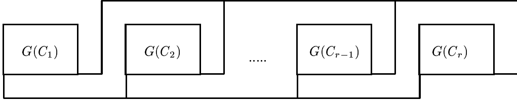
Figure 5: G(\bigvee_{i=1}^r C_i)
