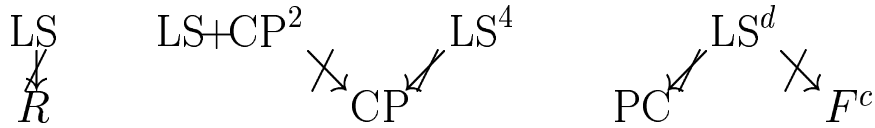
Figure 2: Known separations between semi-algebraic and other proof systems for formulas in DNF (except for PC which is considered for formulas in k -DNF only, i.e., PHP is not a valid counterexample for it): \pi_A \not\rightarrow \pi_B means that there is a formula that has polynomial-size \pi_A proofs and has no polynomial-size \pi_B proofs. F^c denotes constant-depth Frege systems. See Fig. 1 for other notation. Only the strongest separations relevant to semi-algebraic systems are shown. The leftmost separation is due to PHP (the positive part is proved in [Pud99], the negative part is proved in [Hak85]). The counterexample for CP (which provides the two separations in the middle) is given by the clique-coloring tautologies (resp., Theorem 4.1 and [Pud97]). The two rightmost separations are due to Tseitin's formulas (resp., Theorem 6.1 and [BS02]). Note that the knapsack problem is not a valid counterexample because it is not a translation of a formula in DNF.
