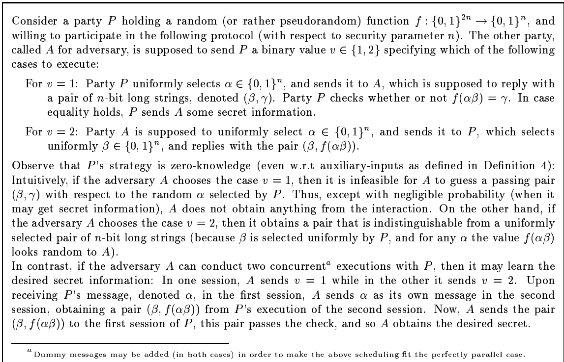
Figure 3: A counter-example (adapted from [55]) to the parallel repetition conjecture for zero-knowledge protocols.
