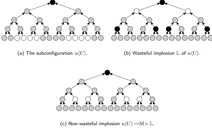
Figure 8: Wasteful and corresponding non-wasteful imposition according to condition 3.
