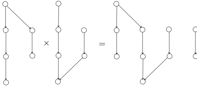
Figure 1: A disconnected product
