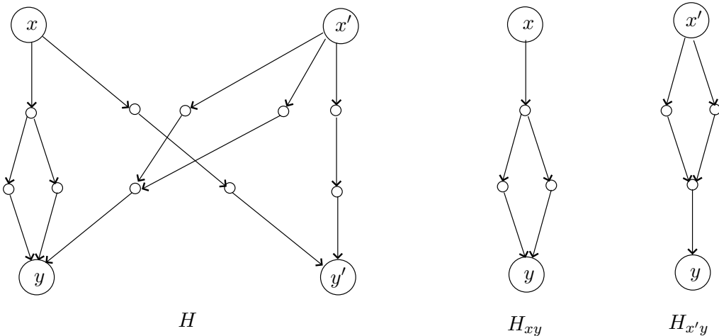
Figure 3: The graph of Example 5.2
