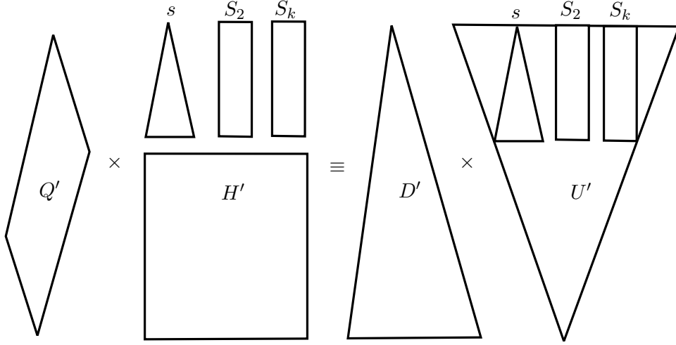
Figure 9: Q'H' \equiv D'U'
