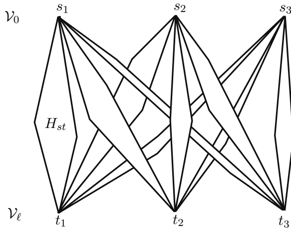
Figure 10: Fully disjoint case
