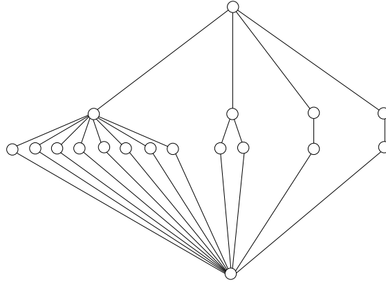
Figure 2: The graph H_1 in Example 2.2
