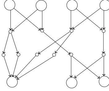
Figure 5: A Lovász-good H
