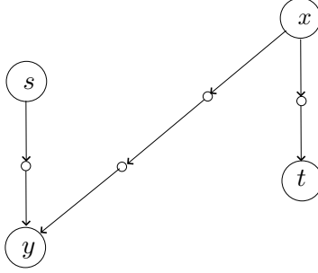
Figure 4: An easy H with no st path
