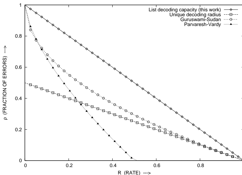
Figure 1: Error-correction radius \rho plotted against the rate R of the code for known algorithms. The best possible trade-off, i.e., capacity, is \rho = 1 - R , and our work achieves this.
