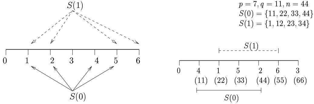
Figure 2: Proof of Prop 12
