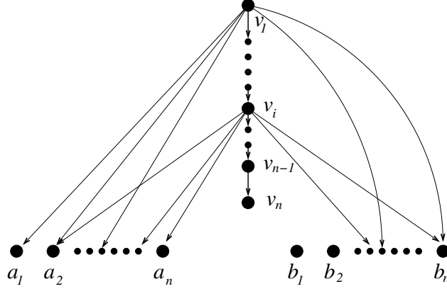
Figure 3: A scheme of the construction used in the proof of Theorem 13.
