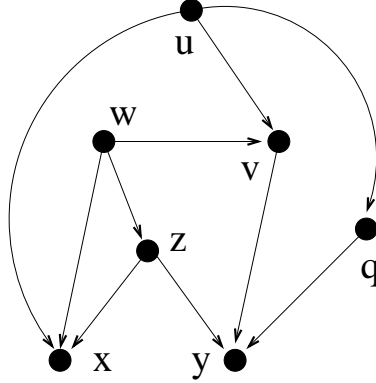
Figure 1: A dag with 7 vertices. The LCA of vertices x and y are both vertex u and vertex z ; vertex w is a common ancestor of x and y but it is not the LCA of x and y . There is no common ancestor of vertices w and q .
