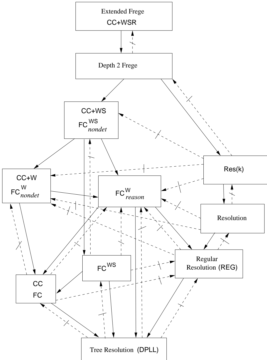
Figure 8: The Relative Complexity of Caching Proof Systems. Solid arcs denote p-simulation. Dashed arcs with slashes denote exponential separation.
