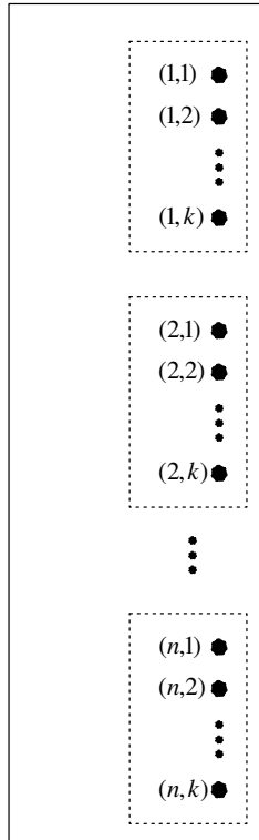
Figure 1: Generator Matchgate \Gamma . We omit all the internal structures. All the kn external nodes are labeled by a pair of integers and they are all on the outer face.
