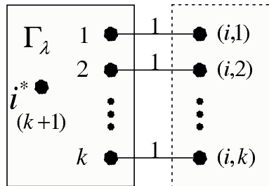
Figure 6: Extend the i -th block of recognizer \Gamma' by a copy of \Gamma_\lambda . We rename the (k+1) -th node of this copy of \Gamma_\lambda as i^* , which is the i -th external node of the new recognizer \widehat{\Gamma}' .
