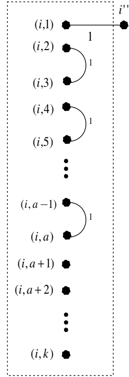
Figure 5: Modify the i -th block of \Gamma when j_i = 1 . All the nodes are viewed as internal in \Gamma_\lambda
