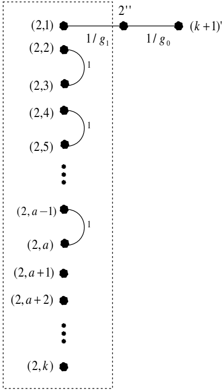
Figure 4: Modify the second block of \Gamma to get the (k+1) -th external node of \Gamma_\lambda
