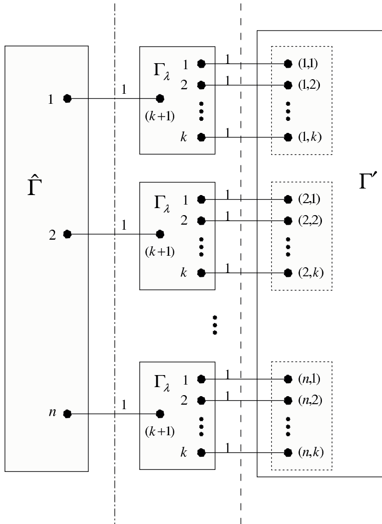
Figure 7: This figure gives an overall picture of our collapse result. When separate the graph from the dashed line (---), we have the original generator \Gamma (left) and recognizer \Gamma' (right) in a size k basis. When separate the graph from the dashed-dotted line (- · - · -), we have the new generator \hat{\Gamma} (left) and recognizer \hat{\Gamma}' (right) in a size 1 basis.
