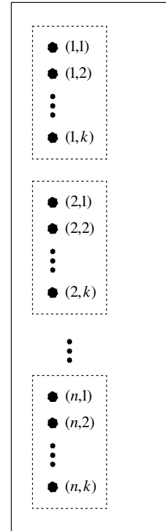
Figure 2: Recognizer matchgate \Gamma' . We omit all the internal structures. All the kn external nodes are labeled by a pair of integers and they are all on the outer face.
