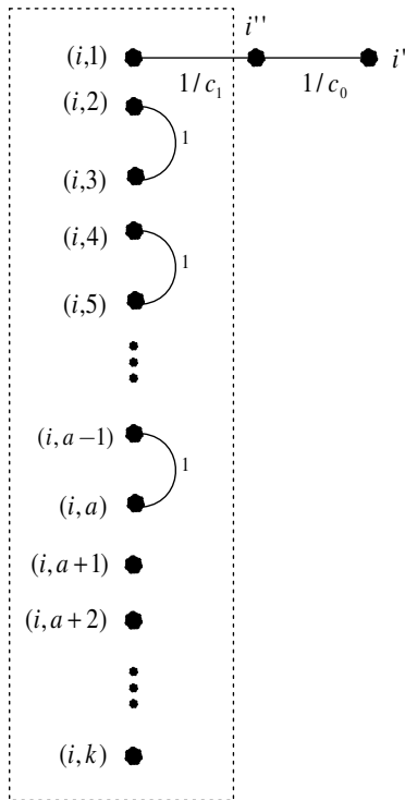
Figure 3: Modify the i -th block of \Gamma to get the i -th external node of \widehat{\Gamma}
