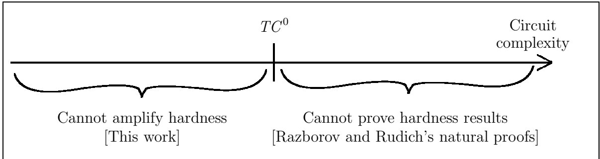
Figure 1: “Lose-lose” reach of current techniques. Recall TC^0 is the class of polynomial-size constant-depth circuits with majority gates.
