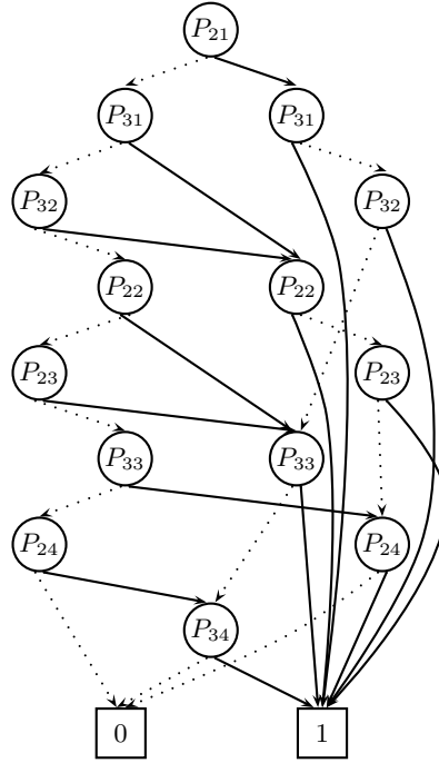
Fig. 4. An OBDD for \bigwedge_{i=2}^3 [\bigvee_{j=1}^4 P_{ij}] \wedge [\neg P_{24} \vee \neg P_{34}] , where P_{21} \prec P_{31} \prec P_{32} \prec P_{22} \prec P_{23} \prec P_{33} \prec P_{24} \prec P_{34} .
