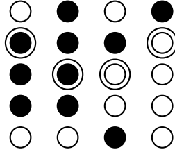
Fig. 3. A 5 \times 4 matrix for \text{PHP}_5 . The black and the white entries represent elements from the sets S_{\prec} and S_{\succ} correspondingly.
