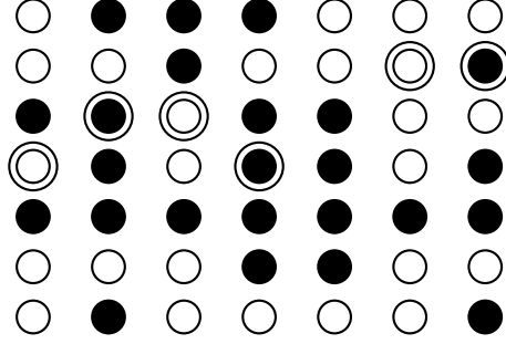
Fig. 2. An example of a 7 \times 7 matrix with entries equally colored black and white.
