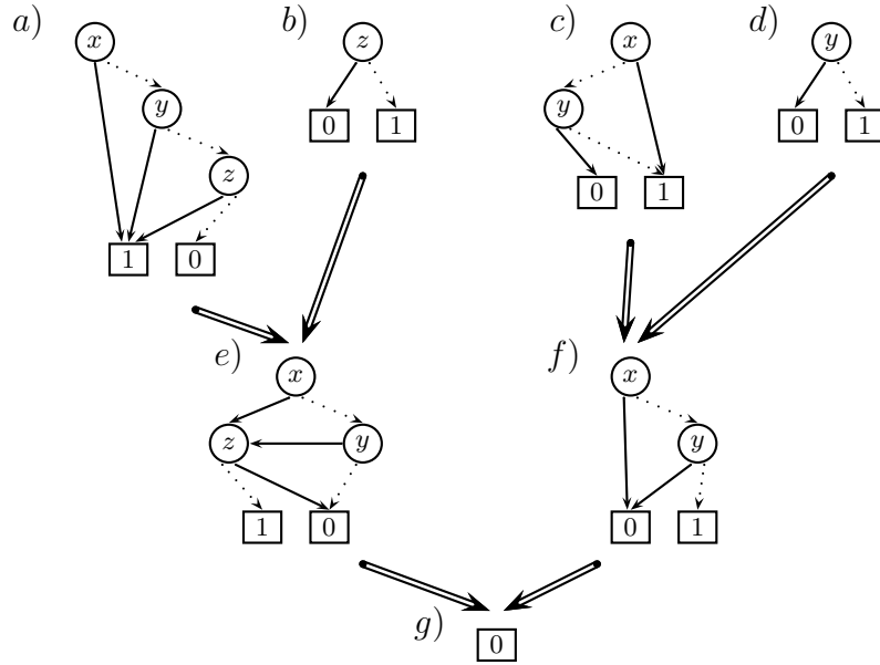
Fig. 1. OBDD refutation of \varphi \equiv (x \vee y \vee z) \wedge (\neg x \vee \neg y) \wedge \neg y \wedge \neg z for the order on variables x \prec y \prec z .
