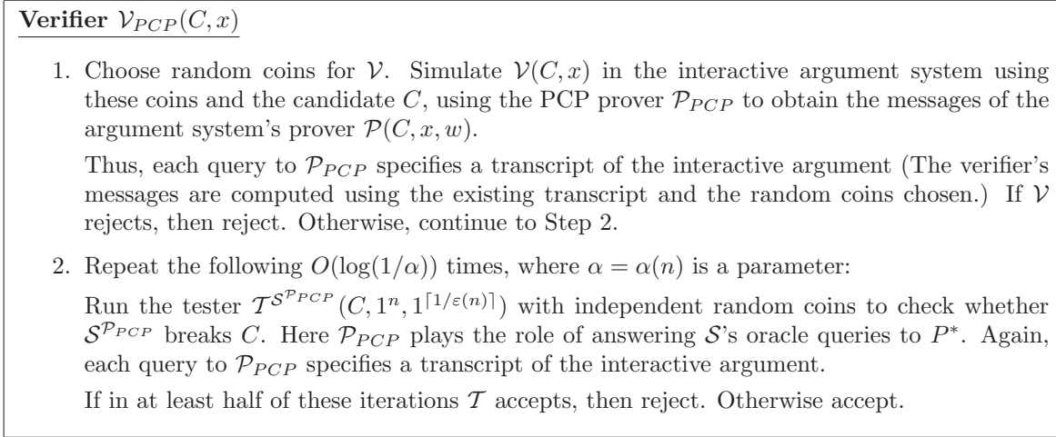
Figure 1: Verifier \mathcal{V}_{PCP}
