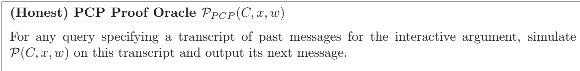
Figure 2: (Honest) PCP Proof Oracle \mathcal{P}_{PCP}
