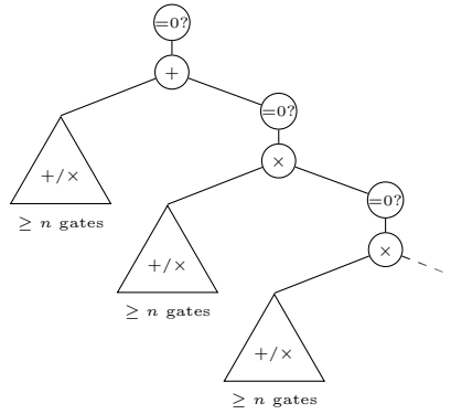
Fig. 1. A circuit violating the small-blob-chains property.
