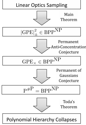
Figure 2: Summary of our hardness argument (modulo conjectures). If there exists a polynomial-time classical algorithm for approximate BOSONSAMPLING, then Theorem 3 says that |GPE|_{\pm}^2 \in BPP^{NP} . Assuming Conjecture 6 (the PACC), Theorem 7 says that this is equivalent to GPE_{\times} \in BPP^{NP} . Assuming Conjecture 5 (the PGC), this is in turn equivalent to P^{\#P} = BPP^{NP} , which collapses the polynomial hierarchy by Toda’s Theorem [60].
