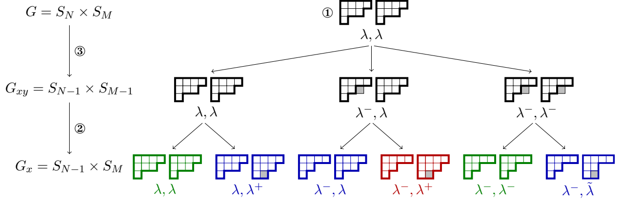
Figure 5: In accordance with our convention, we draw only the part of the diagram below the first row. The condition ① imposes that the two diagrams on top have the same shape. From the first to the second row, one should remove one box to each diagram. When the removed box does not belong to the first row, it is show in light gray. The condition ③ imposes that the left diagram is included into the right one. The condition ② gives the third row of diagrams. Finally we have 3 “generic” types of irreps: case 1 (blue) where the irreps have the same shape; case 2 (green) where the right diagram has one more box; and case 3 (red) where the the right diagram has 2 more boxes.
