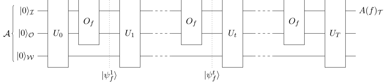
Figure 1: Schematic representation of a quantum algorithm that make use of an oracle O_f , an input register \mathcal{I} , an output register \mathcal{O} , and a register \mathcal{W} for work space.
