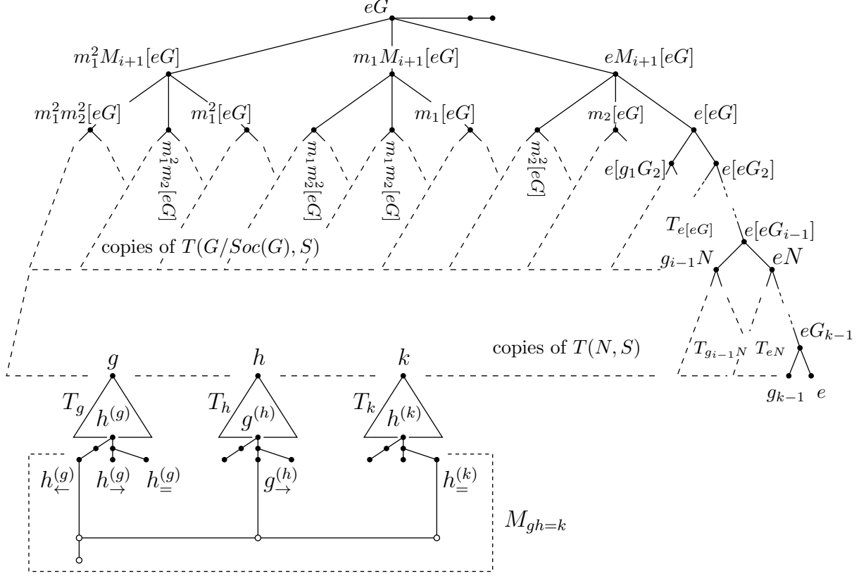
Figure 5: The first two levels in the tree correspond to M . The situation is shown where M is a direct product of two cyclic groups. The tree-levels, from that where e[eG] is contained to that where eN is contained, correspond to G/Soc(G) and consist of copies of T(G/Soc(G), S) , e.g. T_{e[eG]} . The tree-levels from that with eN down to the leaf nodes correspond to N and consist of copies of T(N, S) , e.g. T_{g_{i-1}N}, T_{eN} . Paths from the root to a leaf node correspond to a word mgn \in G , where m \in M, gSoc(G) \in G/Soc(G) and n \in N .
