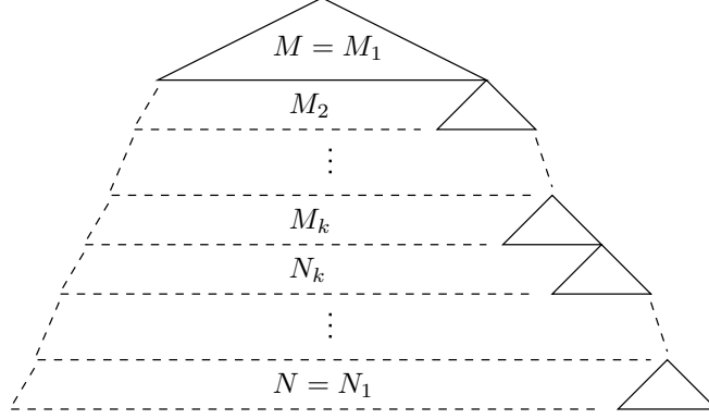
Figure 6: The figure shows schematically the tree construction with recursion.
