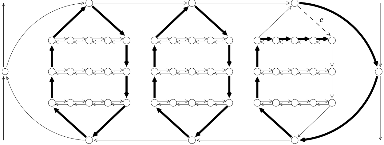
Figure 5: Frame for a mediating outer edge at level \ell = 2 .
