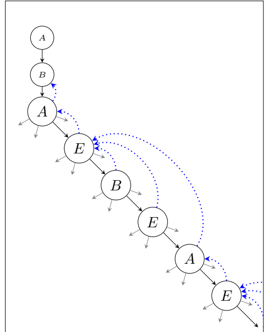
Figure 1: Schematic representation of the nodes in \mathbb{T}^+ (including two initial dummy nodes). The nodes are labeled A , B and E , for Alice, Bob and Eve. The dotted lines show the A_{\text{pred}} relation.
