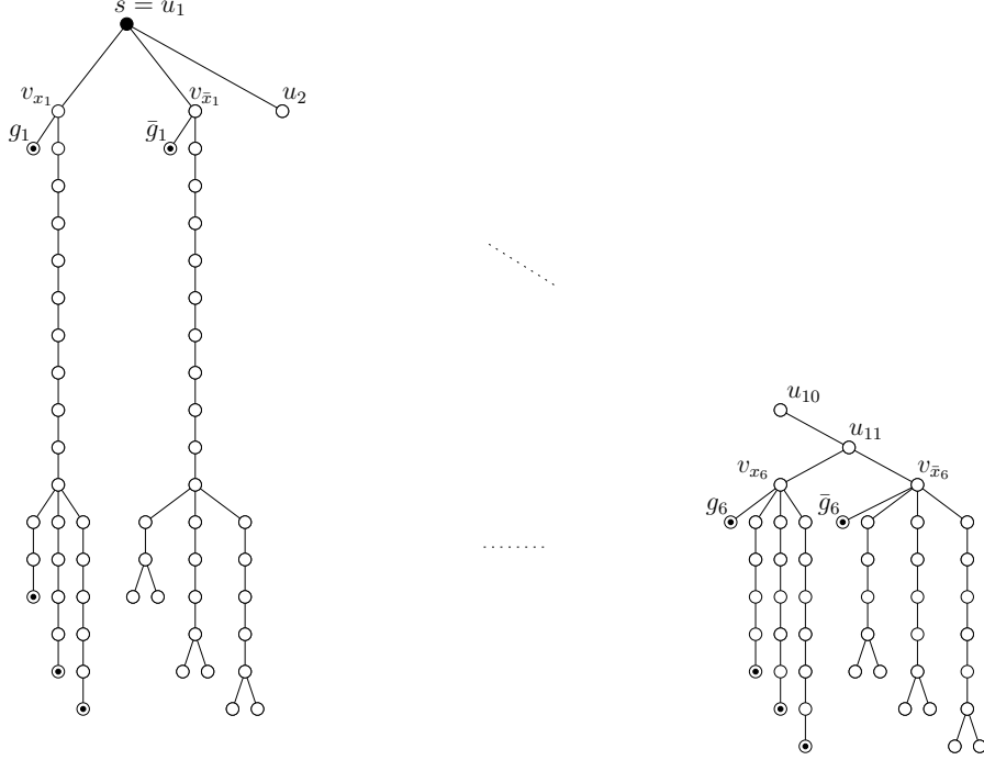
Figure 1: An example of part of a tree constructed from the formula \phi = (x_3 \vee x_4 \vee x_5) \wedge (x_1 \vee x_2 \vee x_3) \wedge (x_2 \vee x_4 \vee x_5) \wedge (x_1 \vee x_3 \vee x_6) \wedge (x_1 \vee x_4 \vee x_6) \wedge (x_2 \vee x_6 \vee x_5) . Guard vertices are represented by a dot within a circle.
