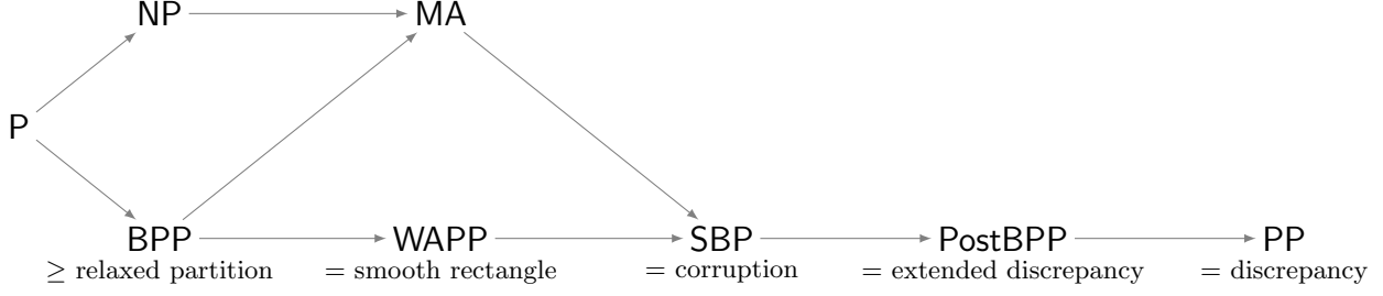
Figure 1: Models and lower bound methods at a glance. Arrows denote class inclusions.
