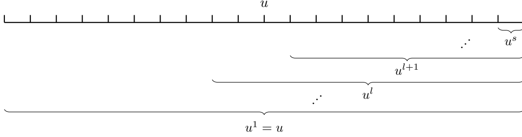
Figure 4: An \alpha suffix decomposition of u of size s . For every l either |u^l| \leq \alpha|u^{l+1}| or u^l = a \cdot u^{l+1} where a is a letter.
