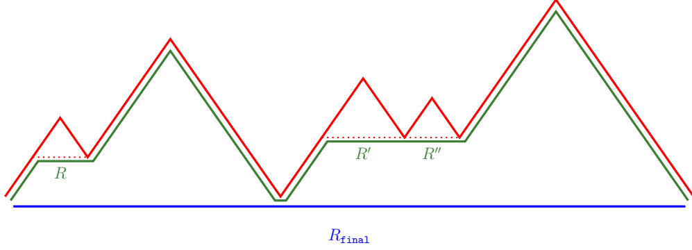
Figure 5: Constructing the words u_0 , u_1 and u_2 as in Lemma 5.8 where \text{Depth}(R_{\text{final}}) = 2
