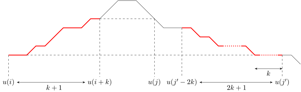
Figure 3: The sampling \mathcal{W}_k(u) from Definition 4.5: sample is in red, dotted parts are for omitted neutral symbols
