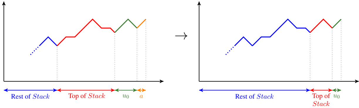
(a) Illustration of lines 10 to 11 from Algorithm 2
