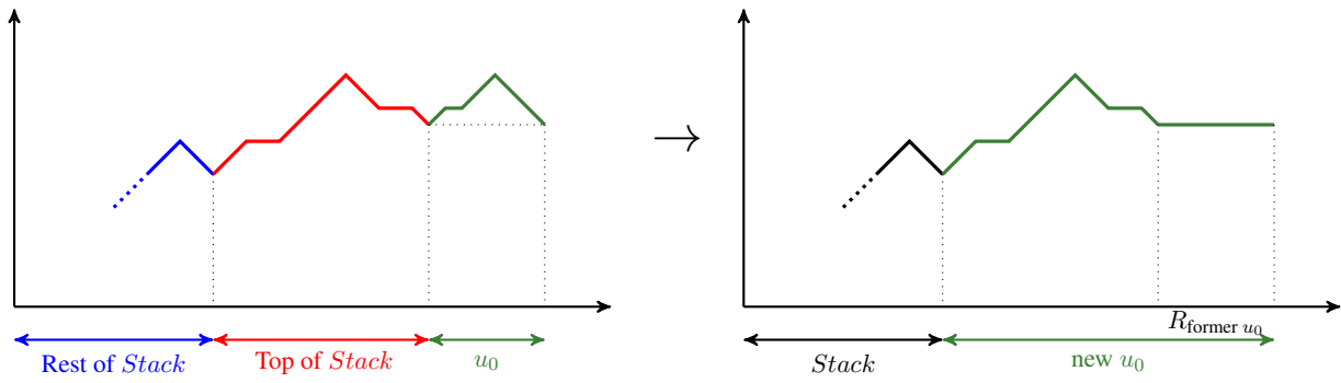
(b) Illustration of lines 13 to 17 from Algorithm 2
