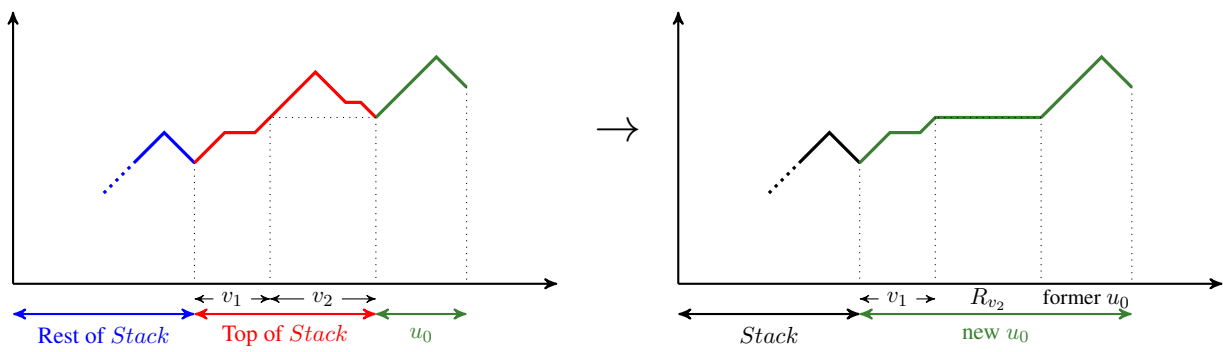
(c) Illustration of lines 18 to 20 from Algorithm 2
