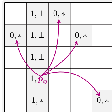
Figure 2: The unambiguous decision tree that defines the Tribes-List function.
