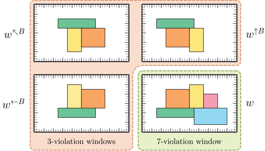
Figure 3: Proof of Claim 9 illustrated. The four windows w , w^{\leftarrow B} , w^{\frown B} , w^{\uparrow B} are rectangles of (x, y) 's. Each (x, y) can be further subdivided according to the private coins (r_A, r_B) of the players. The protocol \Pi_* partitions the extended input space of (xr_A, yr_B) 's into transcript rectangles —above, we have only drawn accepting transcript rectangles (in various colors). For a window w' , the probability \mathbb{P}[\Pi_*|w' = \tau] is simply the area (appropriately scaled) of the transcript rectangle of \tau inside w' . In the proof of Claim 9 , the relevant case is when all of \Pi_*^{\text{acc}}|w^{\leftarrow B} , \Pi_*^{\text{acc}}|w^{\frown B} , \Pi_*^{\text{acc}}|w^{\uparrow B} have roughly the same distribution, say, D (in fact, D := \Pi_*^{\text{acc}}|z ). By the rectangular property of transcripts, this forces \Pi_*|z to overflow onto \Pi_*|w . (Note that \Pi_*^{\text{acc}}|w may contain additional transcripts to those in D , since the acceptance probability is higher.)
