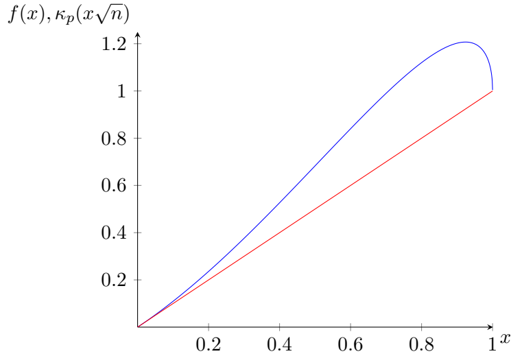
Figure 2: Holmstedt's upper bound (in blue) vs. real behavior of \kappa_p (in red).
