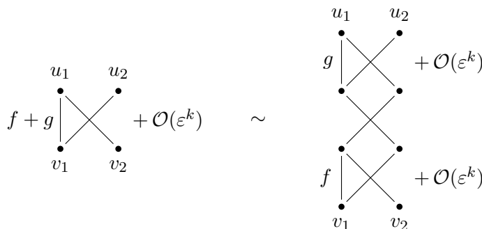
Figure F.1: Addition
