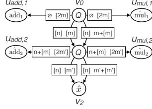
Figure 5: Sum-product circuit and its input for layered circuit of depth 2.
