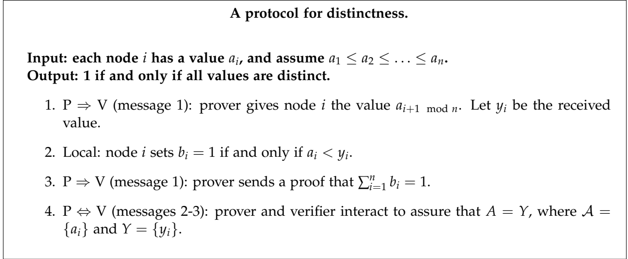
Figure 2: A distributed MAM protocol for checking that each node in the graph has a unique identity i \in [n] .
