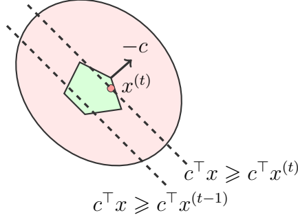
Figure 3.3: A single step of the sliding objective function method.
