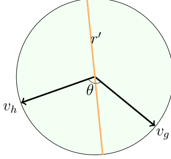
Figure 4.1: A random hyperplane r' separating v_g and v_h .
