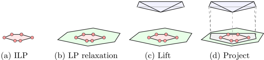
Figure 2.1: The generic form of a lift-and-project procedure. The circles represent the solutions to the ILP. The two-dimensional polygons represent the polytopes in the original variables, while the three-dimensional polyhedron represents the lift, whose two-dimensional shadow is a tightening of the LP relaxation.
