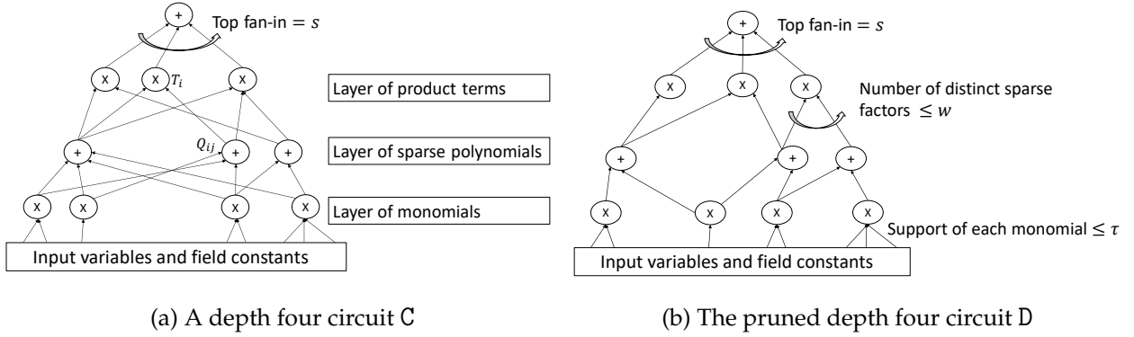
Figure 1: A depth four circuit and its pruned version
