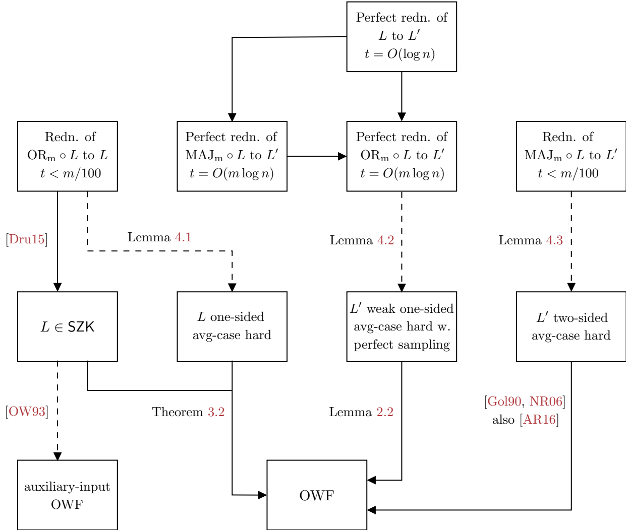
Figure 1: The many paths to One-Way Functions. L and L' are promise problems. The solid arrows denote implications, and the dashed arrows denote implication conditioned on the worst-case hardness of L . In all cases, m and t are polynomials in n , and the reductions lose all but t(n) bits of information on a set of m(n) inputs of size n – that is, t -lossy according to Definition 4.3 (when reducing L to L' , m(n) is set to 1).
