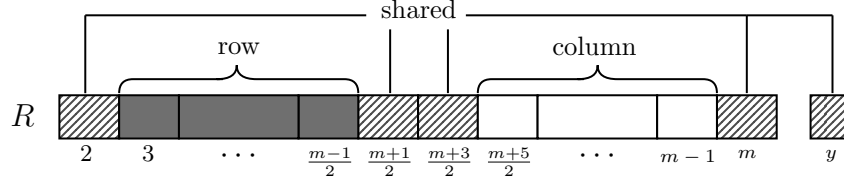
Figure 1: The partition of the randomness of Algorithm 5.5.
