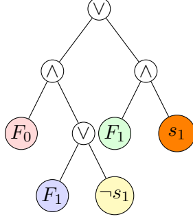
Figure 4: F : a size-optimal hazard-free formula for \text{MUX}_n
