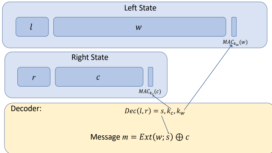
Figure 2: Overview of the construction. Blocks \ell, r come from augmented non-malleable code. The encoder proceeds in steps: first, we randomly sample s, k_w, k_c, w (all independently of the message we are encoding), then we encode s, k_w, k_c using NMC into \ell, r . We then set c = \text{Ext}(w; s) \oplus m , and evaluate \sigma_c as a MAC tag of c on key k_c , and \sigma_w as MAC tag of w on key k_w .
