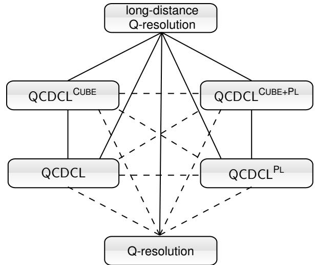
Figure 1: Hasse diagram of the simulation order of QCDCL proof systems. Solid lines represent p-simulations and exponential separations (where the system depicted above is the stronger one). Dashed lines represent separations in both directions (i.e., incomparability).
