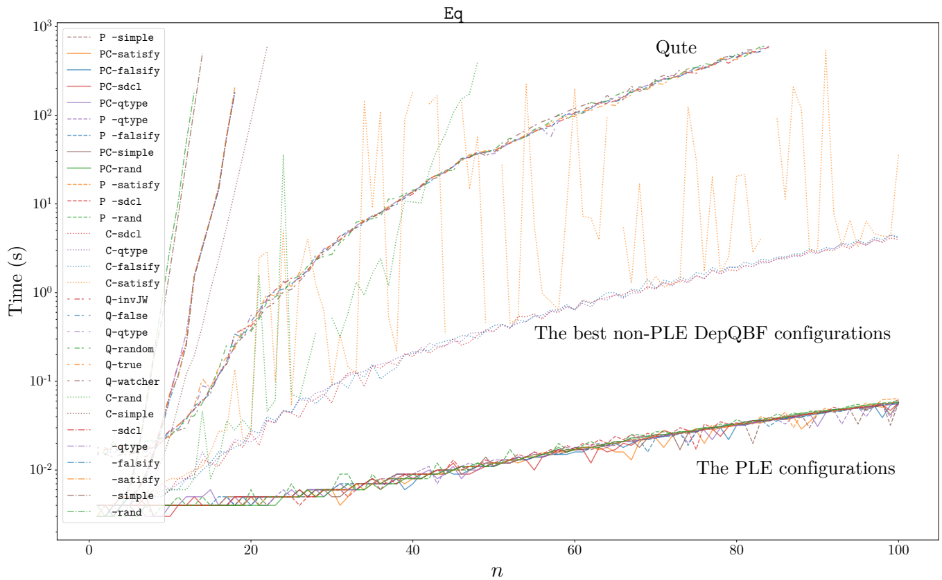
Figure 7: A larger copy of Figure 2.
