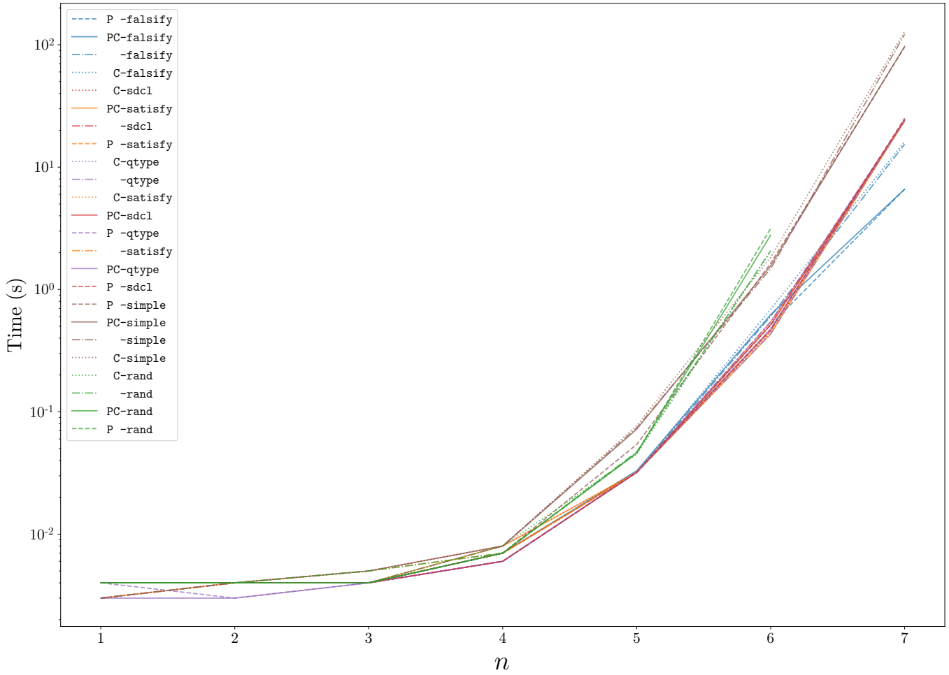
Figure 4: MirrorCR, the same kind of plot as before. We tested the solver on up to n = 10 , but all configurations timed out on n \geq 8 .
