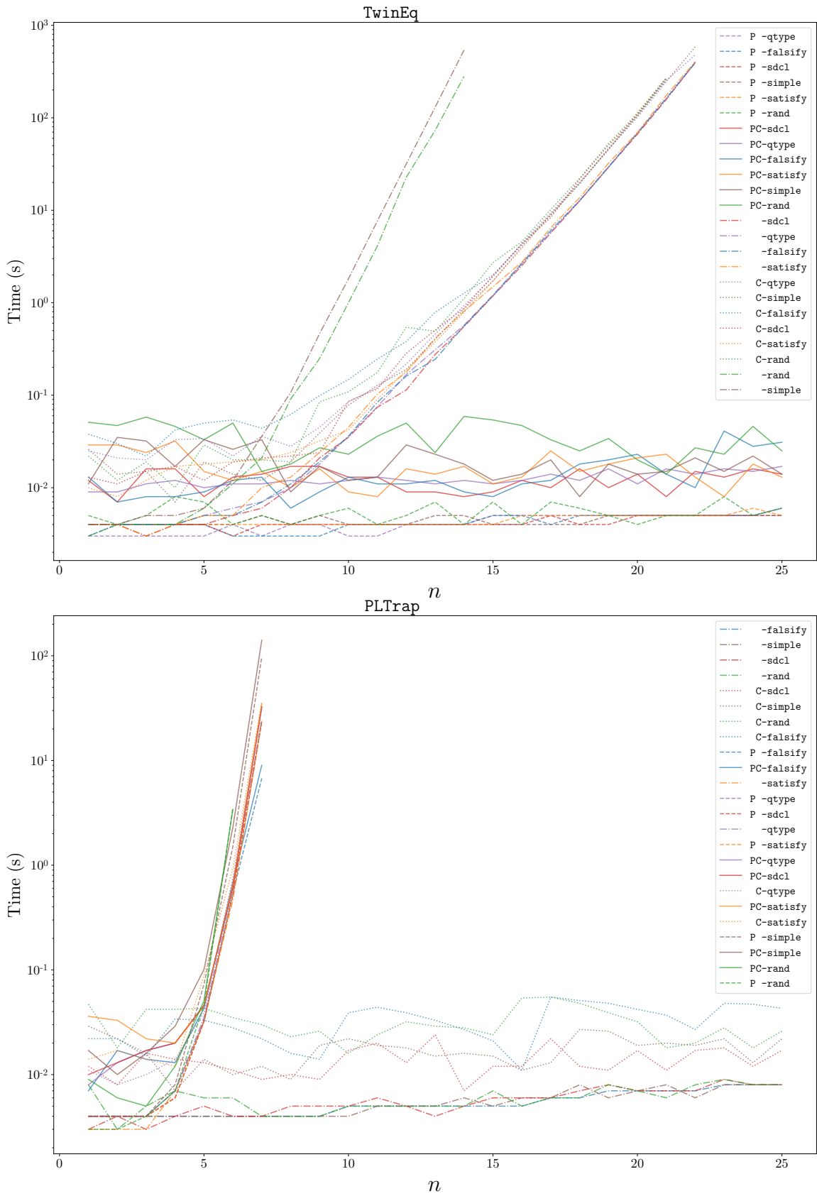
Figure 3: TwinEq (above) and PLTrap (below) formulas documenting Theorem 6.8. Labels indicate whether PLE ("P*") and SDCL ("*C") are on, configurations of one kind have the same line style. The rest of the label is the heuristic; configurations with the same heuristic share colour. Gaps in lines indicate time-outs at 10 minutes. The legend is sorted in descending order of performance.
