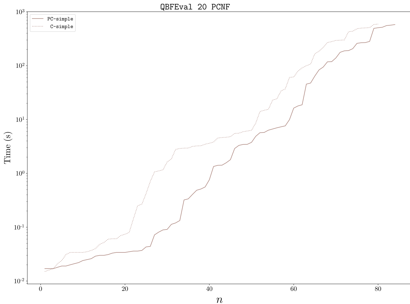
Figure 6: DepQBF on the QBF Evaluation 2020 PCNF Track. Cactus plot; (x, y) means the configuration solved x instances in y seconds. Right and low is better. Lines are labeled like before.
