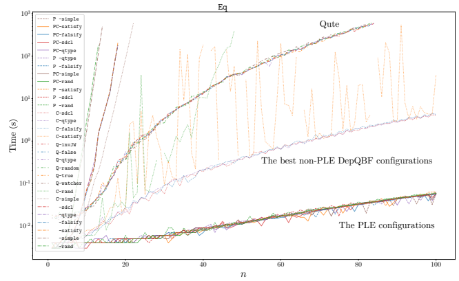
Figure 2: Labels indicate whether PLE (“P*”) and SDCL (“*C”) are on, configurations of one kind have the same line style. Lines for Qute start with “Q”, the remaining lines are for DepQBF. The rest of the label is the heuristic; configurations with the same heuristic share colour. Gaps in lines indicate time-outs at 10 minutes. The legend is sorted in descending order of performance.
