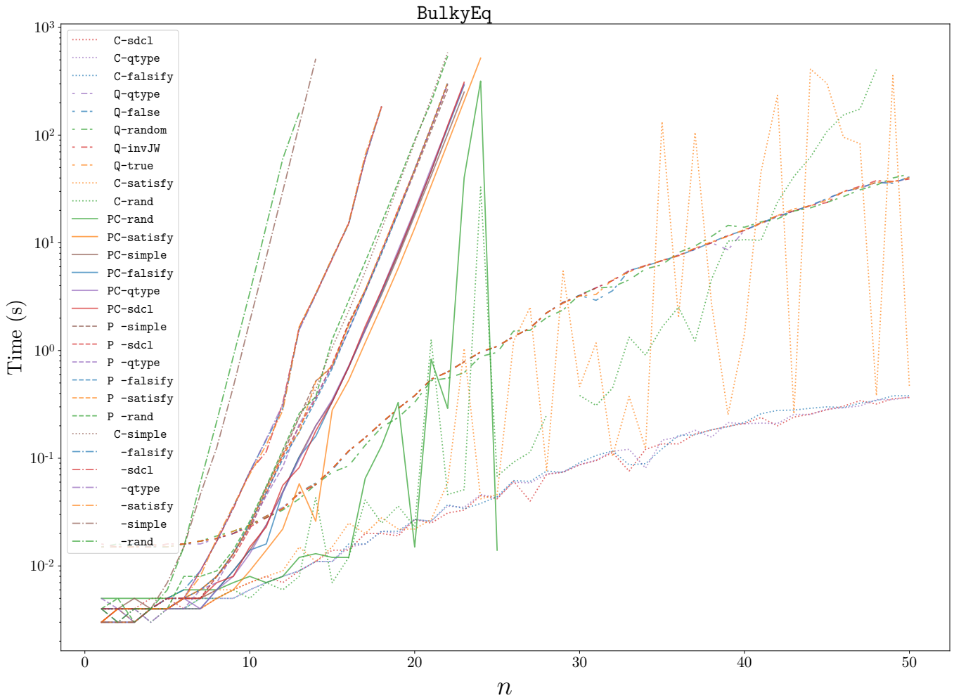
Figure 5: BulkyEq. Lines for Quate start with "Q", the remaining lines are for DepQBF, otherwise the same kind of plot as before.
