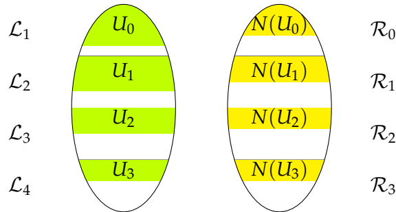
Figure 6: Extracting a threshold from the matching
