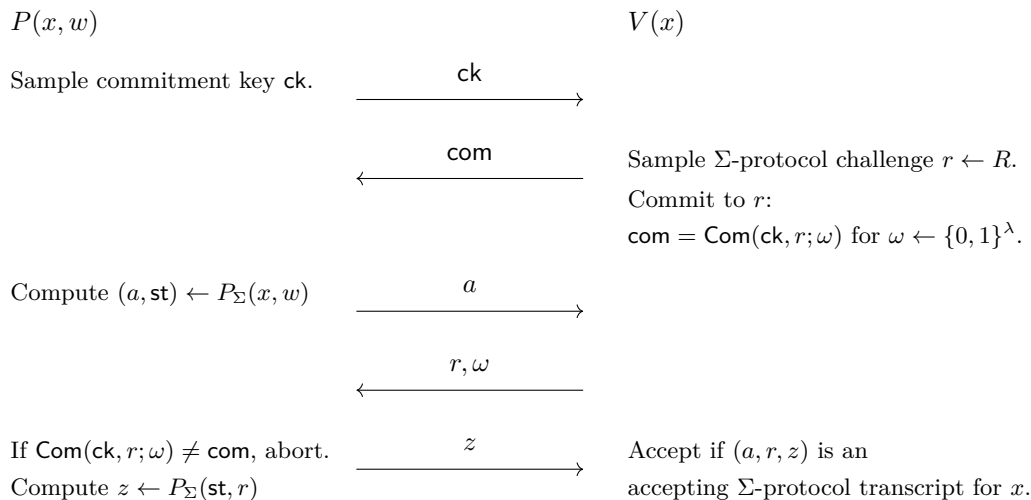
Figure 7: The [GK96] Zero Knowledge Proof System for NP.
