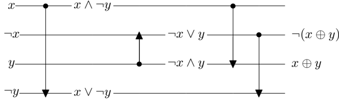
Figure 1: A comparator circuit with 2 inputs, 4 wires and 4 gates. The third wire computes the parity of the two bits.
