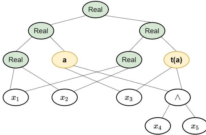
An example of a simple slice formula F . The formula has 5 input bits and one slice gate with fan-in 4.
