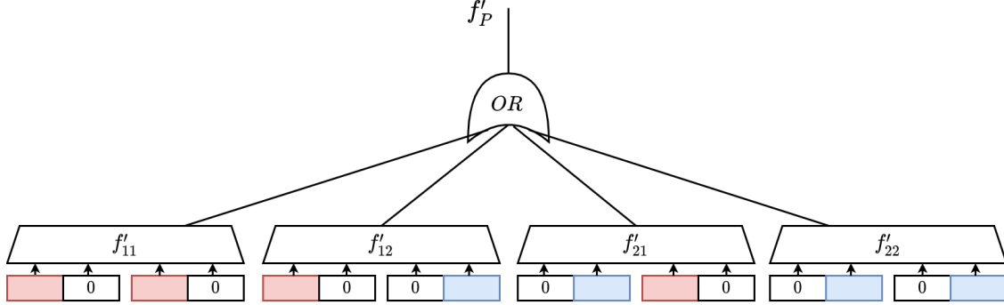
Figure 2: An illustration of Construction 5.21 for a 2-robust realization of a 2-partite function f' : \{\{0, 1\}^A\}^2 \rightarrow \{0, 1\} . Given a partition P of A to a “left” half and a “right” half, we define the function f'_P to be the disjunction of the functions f'_{1,1}, f'_{1,2}, f'_{2,1}, f'_{2,2} , in which different parts of the input are zeroed-out.
