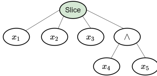
An example of a simple slice formula F . The formula has 5 input bits and one slice gate with fan-in 4.
