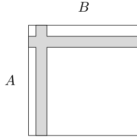
Figure 3: The local view at v from Claim 13. There are at most d_1 \leq \Delta^\gamma rows and d_1 columns (shaded) that are shared with local views from exceptional vertices of S . All other rows and columns are shared with normal vertices of S , and differ from a codeword of C_B or C_A on at most \Delta^{1/2-\varepsilon}/\delta coordinates.
