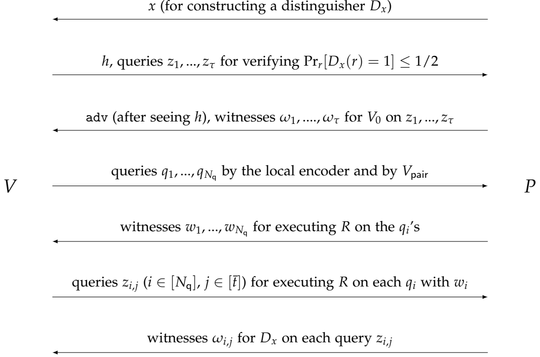
Figure 1: An illustration of the \text{MATIME}^{\llbracket \equiv \rrbracket} protocol for f_\ell in the reconstruction argument. The verifier V is on the left-hand side and the prover P is on the right-hand side, and observe that the prover speaks first.
