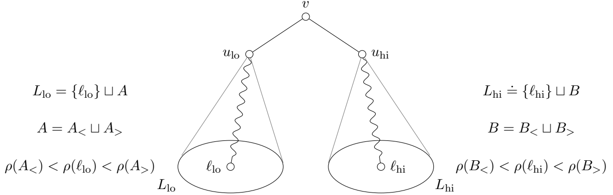
Figure 9: Sensitivity analysis for binary trees
