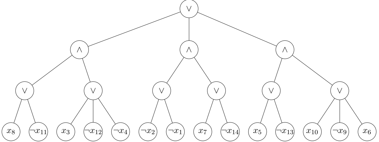
Figure 2.4: A depth-3 read-once \mathbf{AC}^0 formula.
