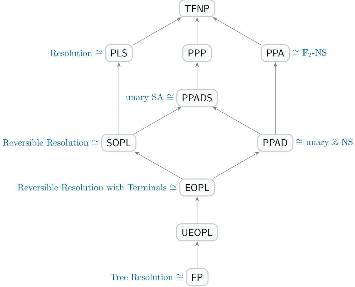
Figure 1: Class inclusion diagram for TFNP. An arrow A \rightarrow B means A \subseteq B relative to all oracles. In the black-box model some classes can be captured using propositional proof systems, as indicated in blue. Above SA refers to the Sherali-Adams proof system [SA94], NS refers to the Nullstellensatz proof system [BIK + 94], and “unary” refers to the fact that we measure size by the sum of all coefficients occurring in the proof.
