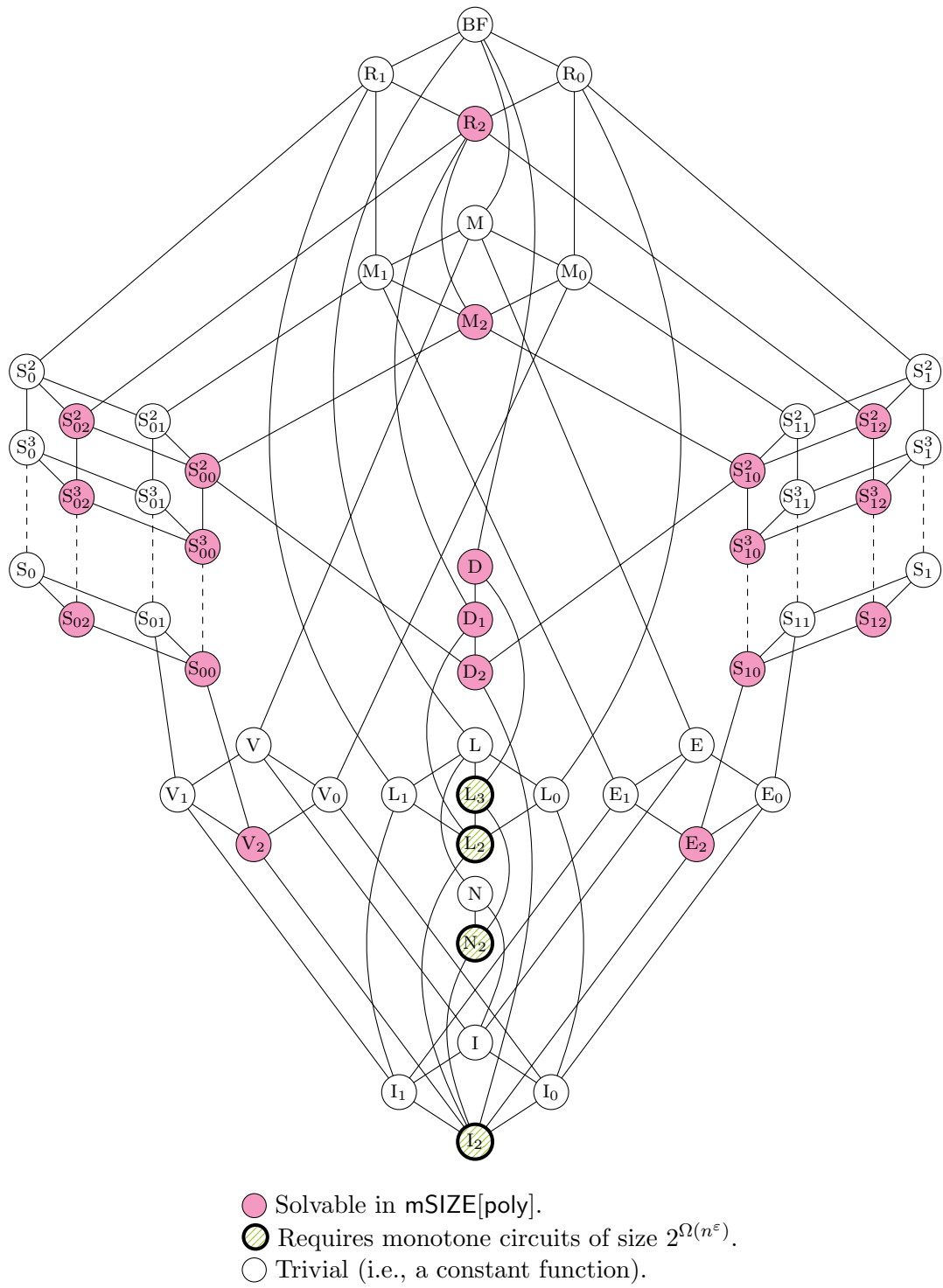
Figure 2: Illustration of Theorem 5.8. The vertices are colored with the monotone circuit size complexity of deciding CSPs whose set of polymorphisms corresponds to the label of the vertex.
