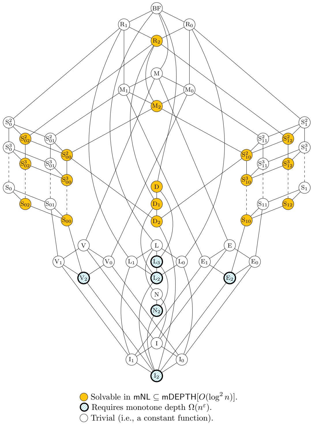
Figure 3: Illustration of Theorem 5.12. The vertices are colored with the monotone circuit depth complexity of deciding CSPs whose set of polymorphisms corresponds to the label of the vertex.
