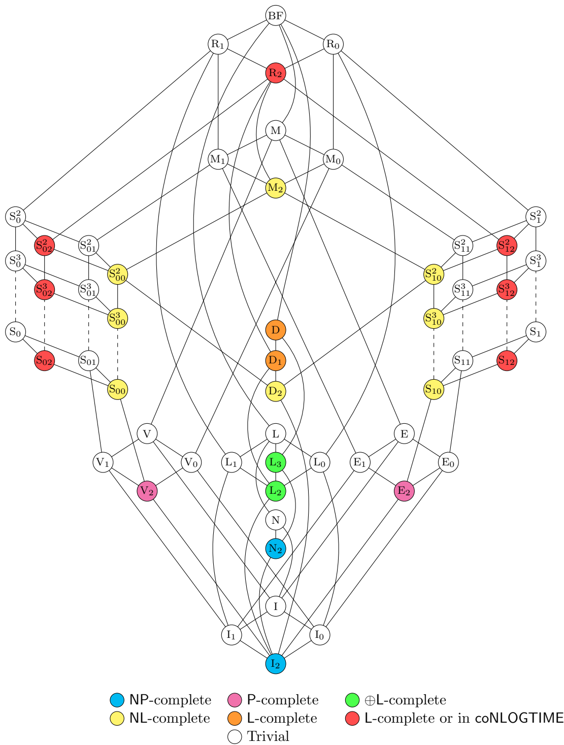
Figure 1: Graph of all closed classes of Boolean functions. The vertices are colored with the complexity of deciding CSPs whose set of polymorphisms corresponds to the label of the vertex. Trivial CSPs are those that correspond to constant functions. Every hardness result is proved under \leq_m^{\text{AC}^0} reductions. See Theorem 5.6 for details. A similar figure appears in [ABI + 09, Figure 1].
