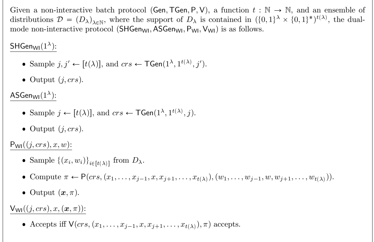
Figure 2: Template for constructing dual-mode NISWI protocols from non-interactive batch protocols
